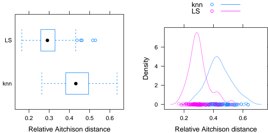
Figure 4: Left: Default plot of results from a simulation study with one missing value rate, in this example obtained by plot(results, xlab = "Relative Aitchison distance") . Right: Kernel density plots of the simulation results, obtained by simDensityplot(results, alpha = 0.6, xlab = "Relative Aitchison distance") .
