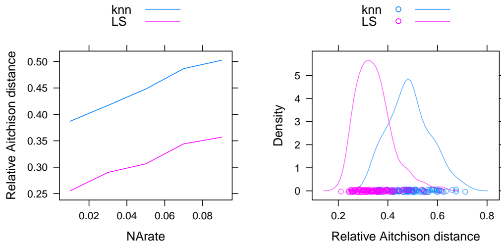
Figure 5: Left: Default plot of results from a simulation study with multiple missing value rates, in this example obtained by plot(results, ylab = "Relative Aitchison distance") . Right: Kernel density plots of the simulation results for a specified missing value rate (7%), obtained by simDensityplot(results, NArate = 0.07, alpha = 0.6, xlab = "Relative Aitchison distance") .
